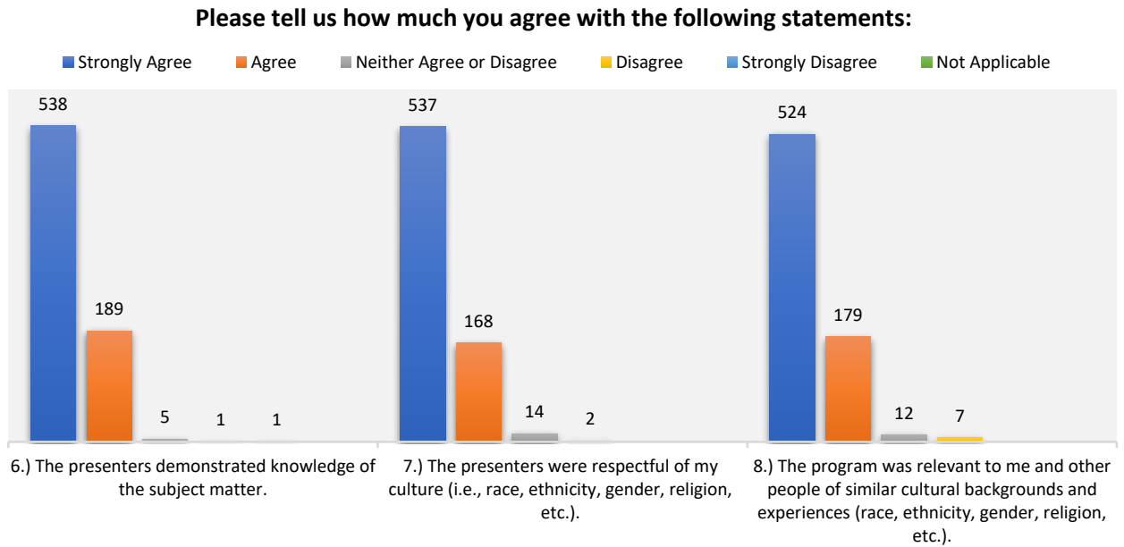
Figure 23. Training Quality
