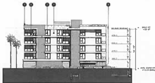
C. WEST ELEVATION
