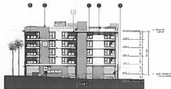
D. EAST ELEVATION
