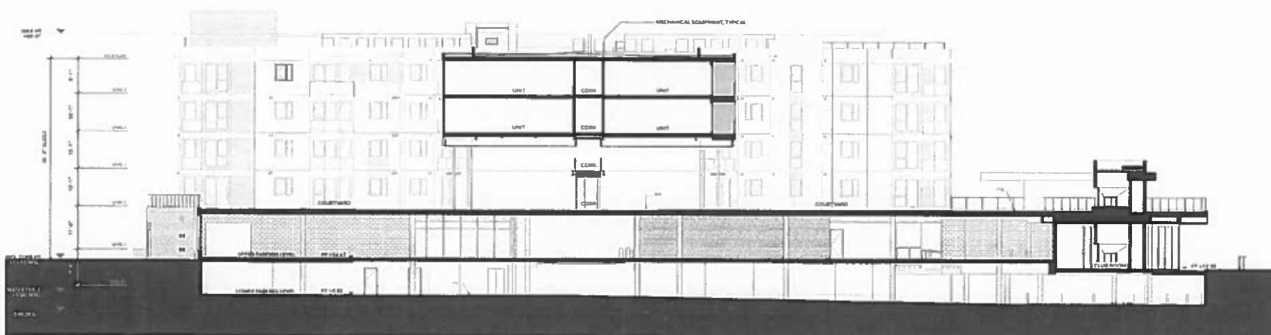
BLDG 3 - ENLARGED SECTION (B)
