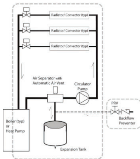
FIGURE U 9.2.1(1) 1,2 EXAMPLE OF A CLOSED-LOOP SYSTEM WITH DIAPHRAGM TYPE EXPANSION TANK (SIMPLIFIED SCHEMATIC)
