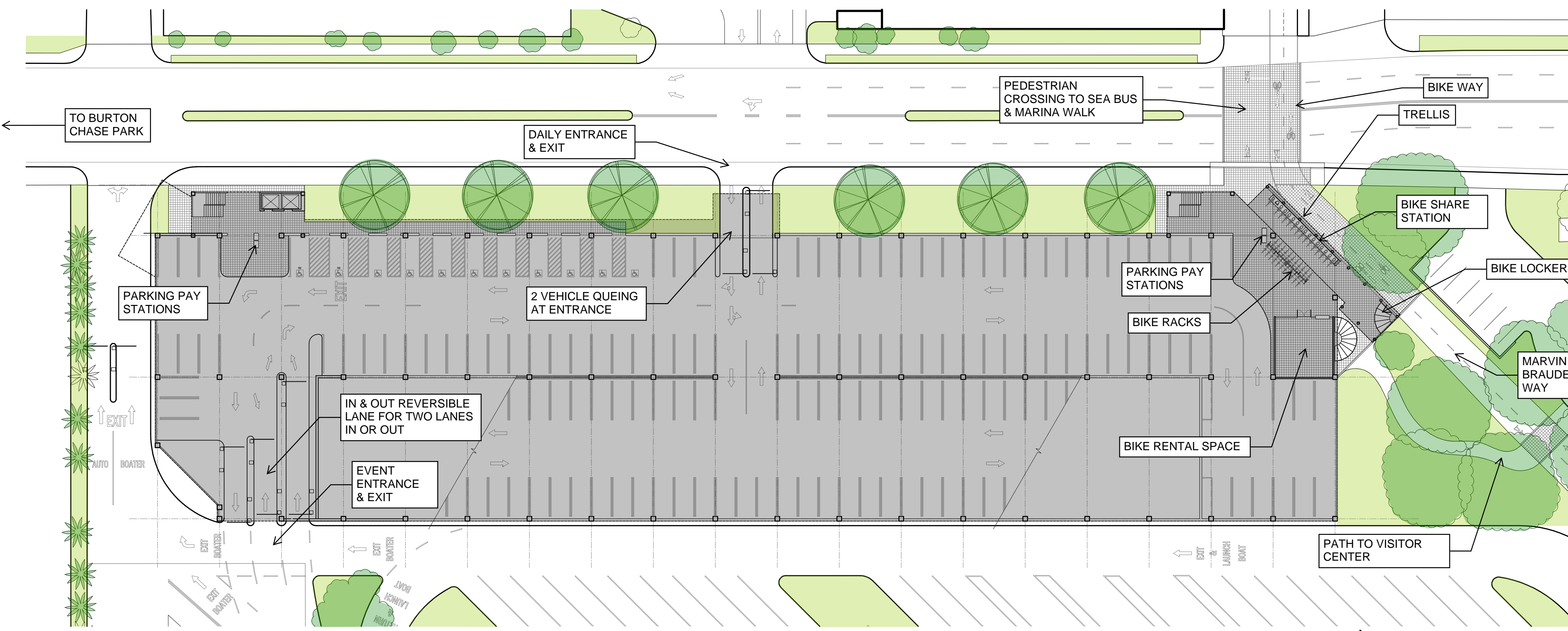
FIRST LEVEL PLAN
