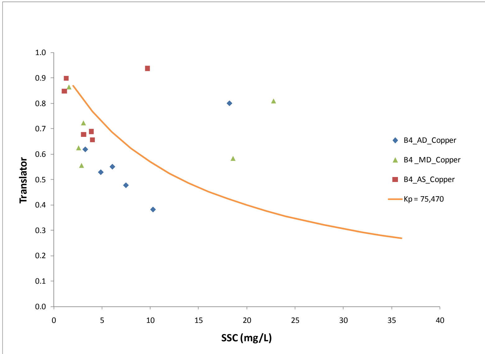
Figure E.9. Copper Translators versus SSC for MdrH-B4 Samples with Various Partitioning Coefficients.
