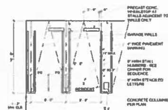
TYPICAL STANDARD PARKING STALL
