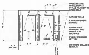
TYPICAL COMPACT PARKING STALL NON-RESIDENTIAL FOR GUEST & MARINA
