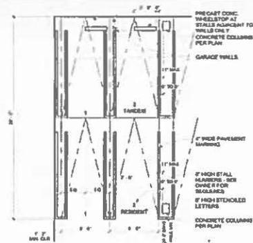
TYPICAL TANDEM PARKING STALL FOR RESIDENTIAL USES
