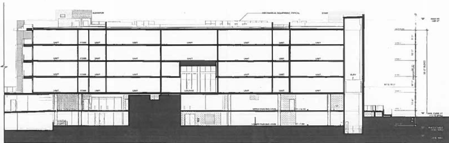
BLDG 3 - ENLARGED SECTION (A) 1/8" = 1'-0"
