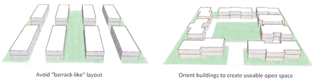
Figure 3-5: Site Layout to Create Usable Space
