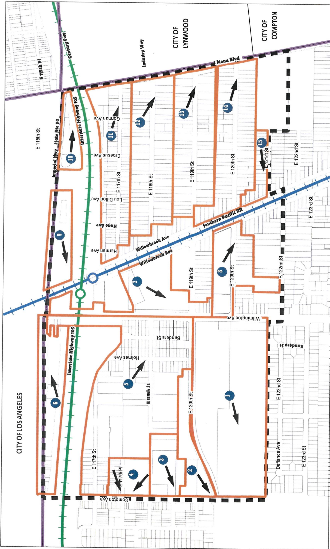
Figure 6-4 Tributary Areas for Calculating Sewer Demand
