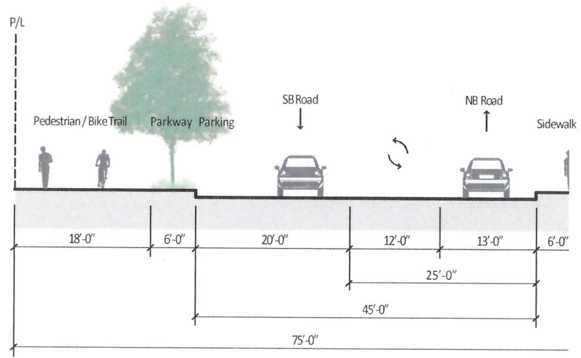
Figure 4-3: Proposed Mona Boulevard Section
