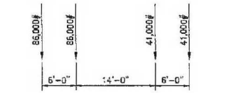
MAX. BRIDGE WHEEL LOADS WITH FORKS PERPENDICULAR TO CRANE BRIDGE GIRDERS (STATIC).
