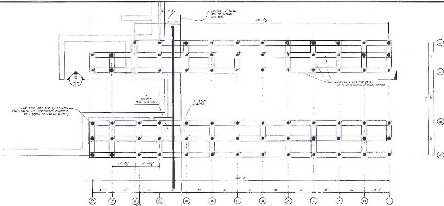
FOUNDATION PLAN SCALE 1"=30'
