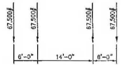
MAX. BRIDGE WHEEL LOADS WITH FORKS PARALLEL TO CRANE BRIDGE GIRDERS (STATIC).
