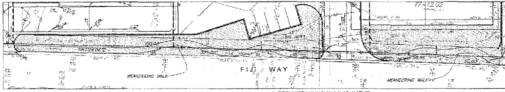
ALTERNATE WALKWAY ALIGNMENT
