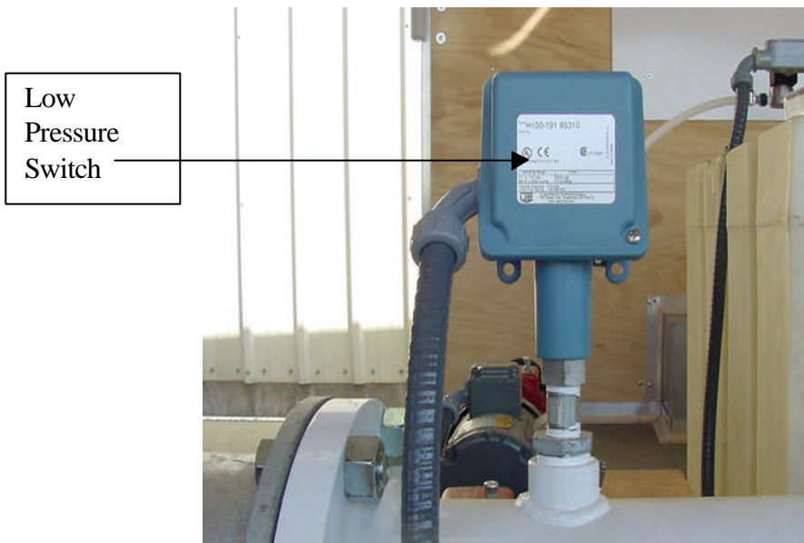
Figure 4: Pressure switch
