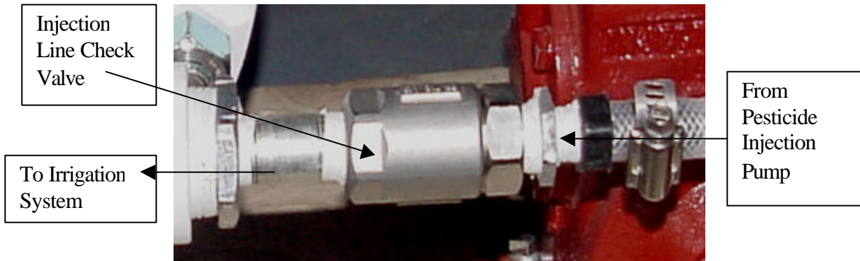
Figure 2: Quick-closing check valve on pesticide injection line
